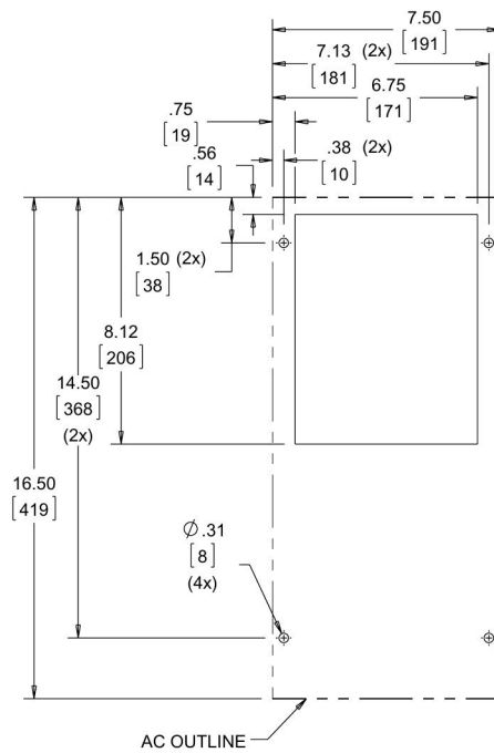
Cutout Dimensions (Externally Mounted)
